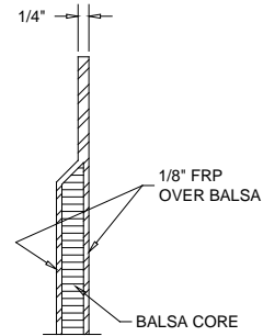
CROSS SECTION GATE WITH Balsa
